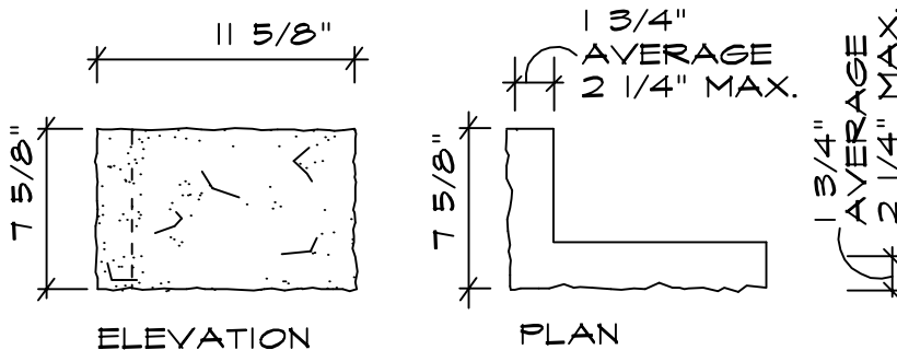
QUOIN PROFILE
